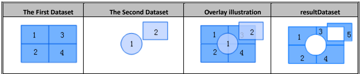
Diagram 7 Symmetric Difference Operation Diagram
