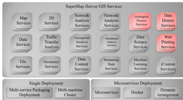
SuperMap iServer Service System Architecture
