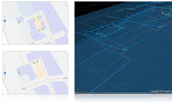
Indoor Navigation
