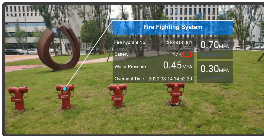
AR Recognition
